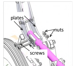
pic. 11.1: Posterior part depth adjustment
