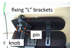
pic. 22: Detachable mechanism
