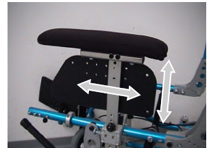
pic.15.2: Depth/height adjustment
