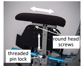
pic. 15.1: Armrest adjustment
