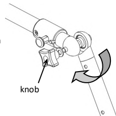
pic. 13.3: Paediatric size knee angle adjustment
