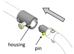
pic. 4.2: Inserting the paediatric size legrest tube
