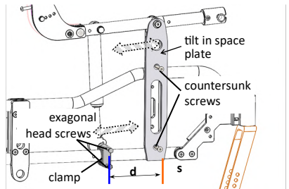
pic. 12.1: Displacement of the seat (Folding model)
