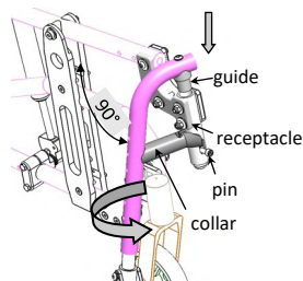
pic. 29: Legrest tube installation/removal
