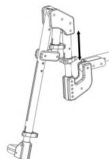
pic. 30: Legrest tube installation/removal
